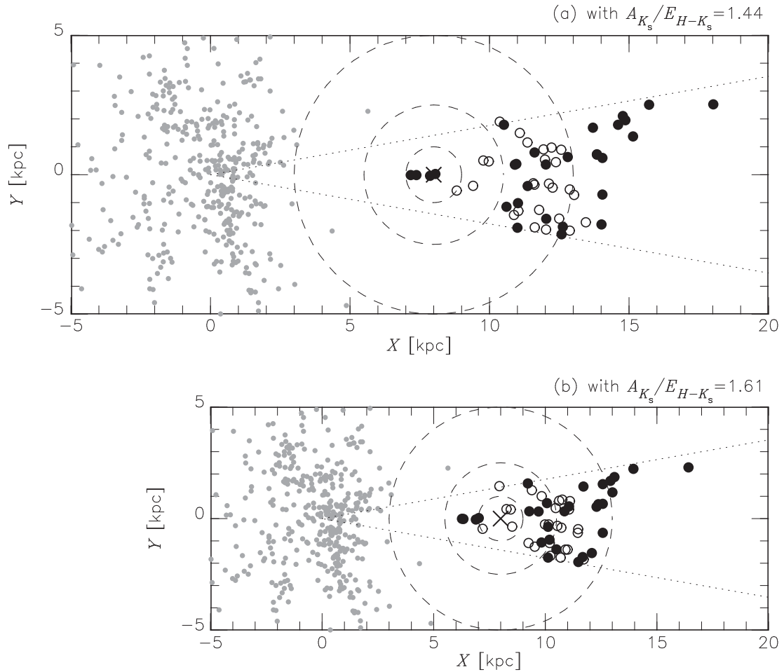
Figure 4. Distribution of Cepheids, ours and those in Dékány et al. (2015a,b) indicated by filled and open circles, respectively, on the face-on view of the Galactic disc. The reddening law by Nishiyama et al. (2006) was used for both sample in the panel (a), while that by Nishiyama et al. (2009) was used in the panel (b). Note the displacement of the four NSD Cepheids from the Centre in (b). If a Cepheid is found in both surveys, a distance obtained with our photometry is used. Grey points show the distribution of previous Cepheids in Fernie et al. (1995). The Sun is located at the origin, and the Galactic Centre is indicated by the cross at an assumed distance of 8 kpc. Dashed circles at 1, 2.5 and 5 kpc from the Galactic Centre are drawn for readers’ convenience. The longitude range of our survey, |l| < 10^\circ , is illustrated by dotted lines.
