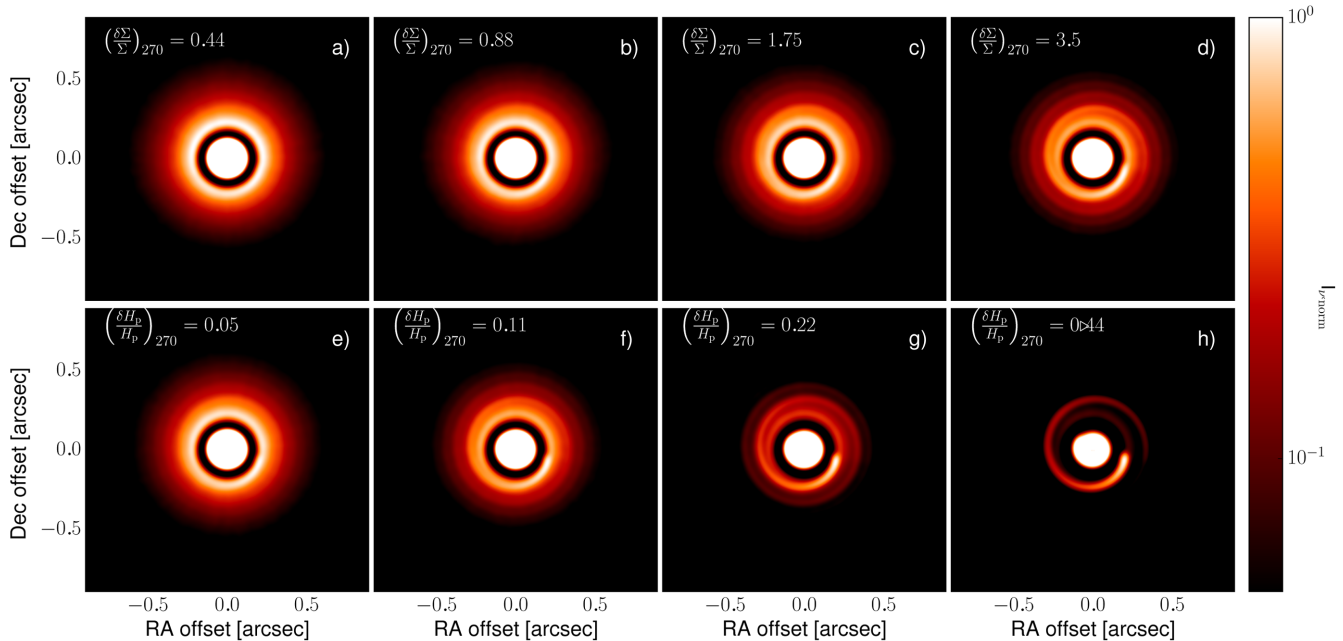
Figure 4. Simulated H -band polarized intensity images with analytic surface density ( a – d ) and pressure scaleheight ( e – h ) perturbations. The images calculated with the radiative transfer code are convolved with a Gaussian PSF with a FWHM of 0.06 arcsec and are normalized to the highest intensity outside of a 0.18 arcsec radius (25.2 au at 140 pc distance) from the central star. The relative change of the perturbed variable at 270^\circ azimuth angle, i.e. along the negative Dec. offset axis, is shown in the top-left corner of each panel. To see the spiral arms in the PSF-convolved images, a perturbation amplitude of a factor of 0.22 and 3.5 above the unperturbed disc is required in the case of pressure scaleheight and surface density perturbations, respectively.
