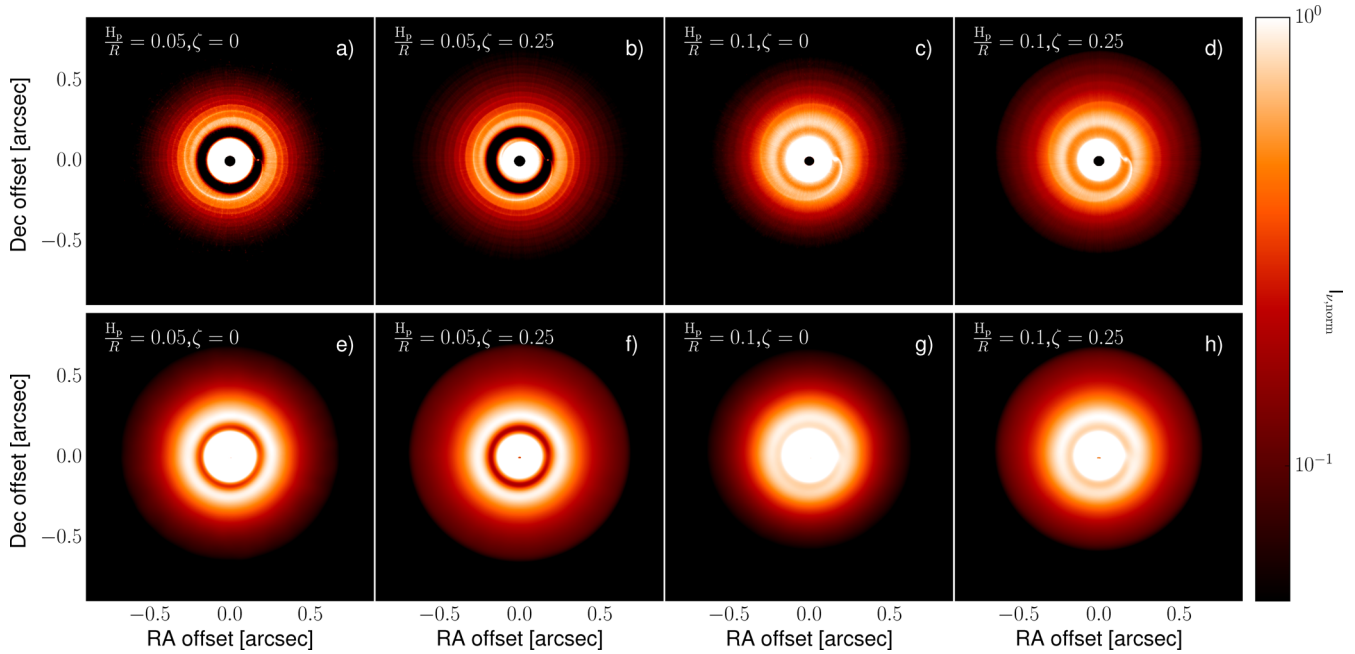
Figure 2. Simulated H -band polarized intensity images with the surface density given by hydrodynamic simulations with a planet-to-star mass ratio of 0.001 for different values of the disc aspect ratio ( H_p/R ) and flare index ( \zeta ). The images are normalized to the highest intensity outside of a 0.18 arcsec radius (25.2 au at 140 pc distance) from the central star. The top row shows images at original resolution as calculated by RADMC-3D , while the bottom row shows the images convolved with a circular Gaussian beam with an FWHM of 0.06 arcsec. While spiral arms are clearly visible in the original, quasi-infinite resolution (top row), no spiral arm is visible after convolving the images with a 0.06 arcsec PSF (bottom row) in any of the images.
