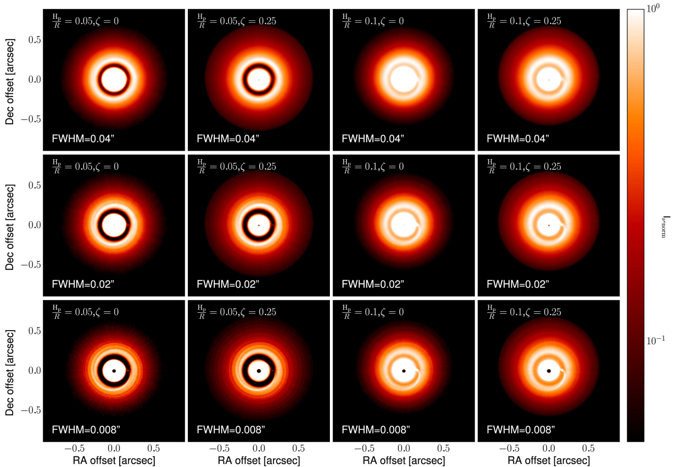
Figure 7. Effect of the spatial resolution on the detectability of spiral arms with pure surface density perturbation. The images are calculated from hydrodynamic simulations for a planet-to-star mass ratio of 0.001. Panels in different columns show models with different values for the aspect ratio ( H_p/R ) and the flaring index ( \zeta ), which is indicated in the top-left corner of each panel. The three rows show the images convolved with Gaussian PSFs representative in size for SPHERE/VLT in the H -band (FWHM = 0.04 arcsec, top row), SPHERE/VLT in the R -band (FWHM = 0.02 arcsec, middle row) and E-ELT in the H -band (FWHM = 0.008 arcsec, bottom row). To detect pure surface density perturbation along the spirals at 140 pc distance, one needs an extreme high spatial resolution, where the FWHM of the PSF is 0.02 arcsec or smaller.
