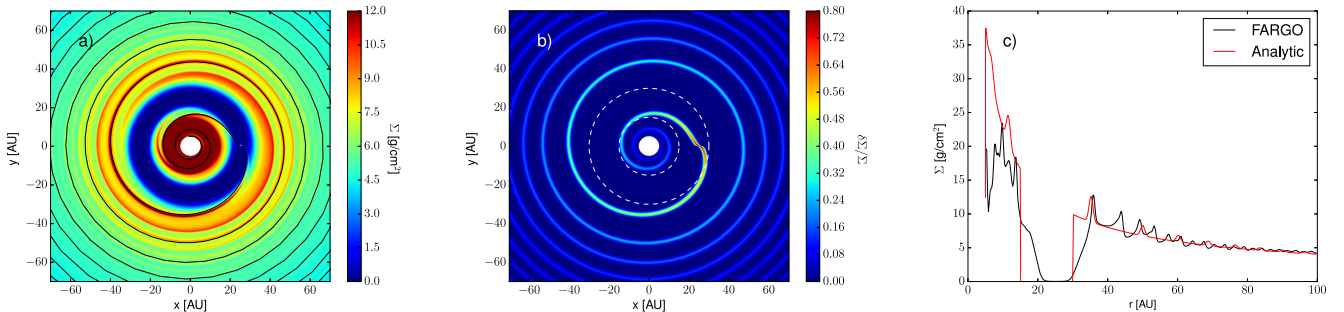
Figure 3. (a) Surface density distribution in the reference hydrodynamical model after 1000 planetary orbits. The black line shows the analytic fit to the spiral wake. (b) Relative surface density perturbation in the analytic model with a spiral perturbation fitted to the reference hydrodynamical model. The white dashed lines mark the inner and outer radius of the applied gap. (c) Surface density as a function of radius along the \phi = 270^\circ azimuth angle (i.e. along the negative y-axis).
