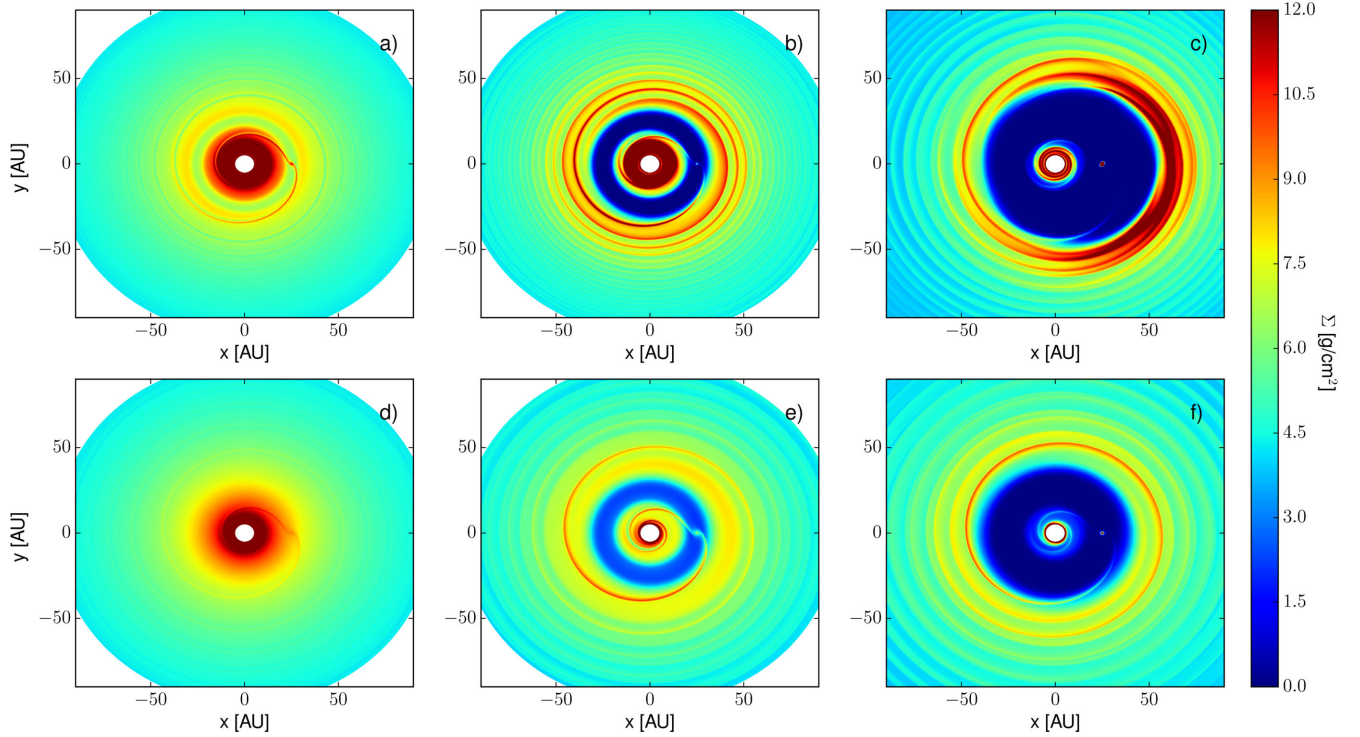
Figure 1. Surface density structure of the disc with an embedded planet for a planet-to-star mass ratio of 6.25 \times 10^{-5} (a,d), 10^{-3} (b,e) and of 10^{-2} (c,f). The upper row shows the surface density for an aspect ratio of H_p/R = 0.05 while the bottom row for H_p/R = 0.1 . The strength and the number of the spirals increases for higher planetary masses and decreases for higher aspect ratio. The spirals become also more open for higher aspect ratios.
