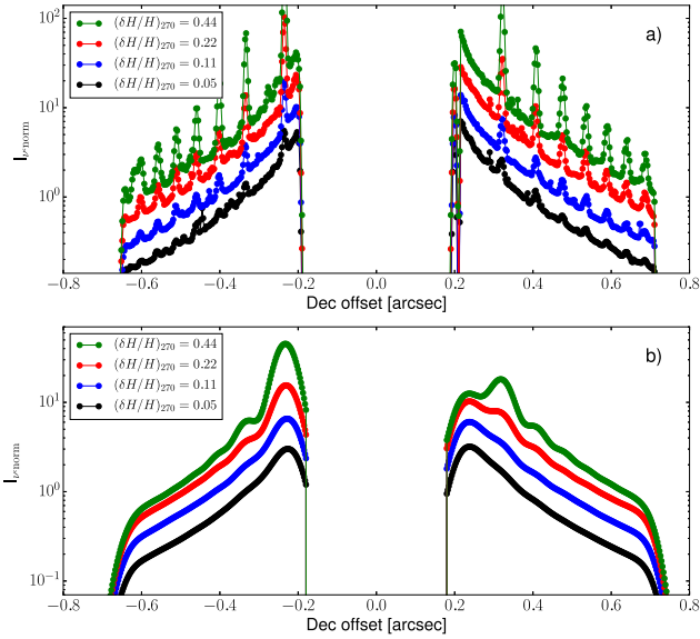
Figure 6. Cross-section of the calculated images with different pressure scaleheight perturbations at original resolution, as calculated by RADMC-3D (Panel a), and after convolved with a 0.06 arcsec circular Gaussian PSF (Panel b).
