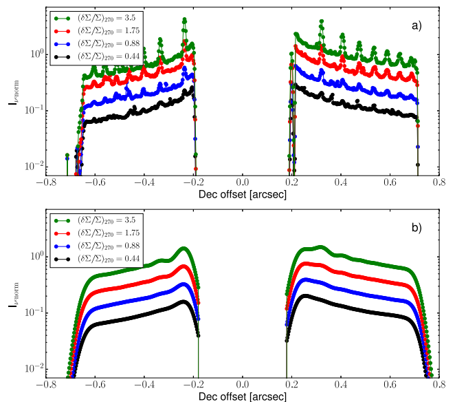
Figure 5. Cross-section of the calculated images with different surface density perturbations at original resolution, as calculated by RADMC-3D (Panel a), and after convolved with a 0.06 arcsec circular Gaussian PSF (Panel b).
