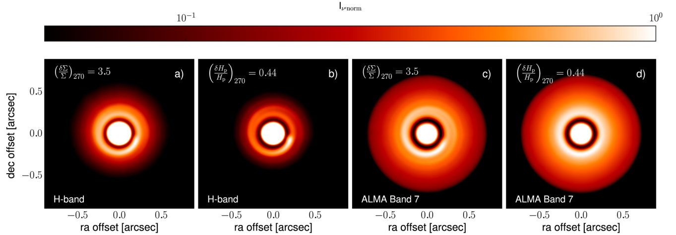
Figure 8. Observability of spirals by surface density (Panels a, c) and pressure scaleheight (Panels b, d) perturbation in NIR polarized intensity (Panels a, b) and submillimetre thermal emission (Panels c, d). The images calculated by the radiative transfer code are convolved with a circular Gaussian kernel with an FWHM of 60 milli-arcsecond. For surface density perturbation the contrast between the spiral and the background disc is the same in the NIR scattered light as in the submillimetre. In contrast, pressure scaleheight perturbation that cause similar amplitude signatures in NIR scattered have extremely weak, practically unobservable, signature in the submillimetre continuum.
