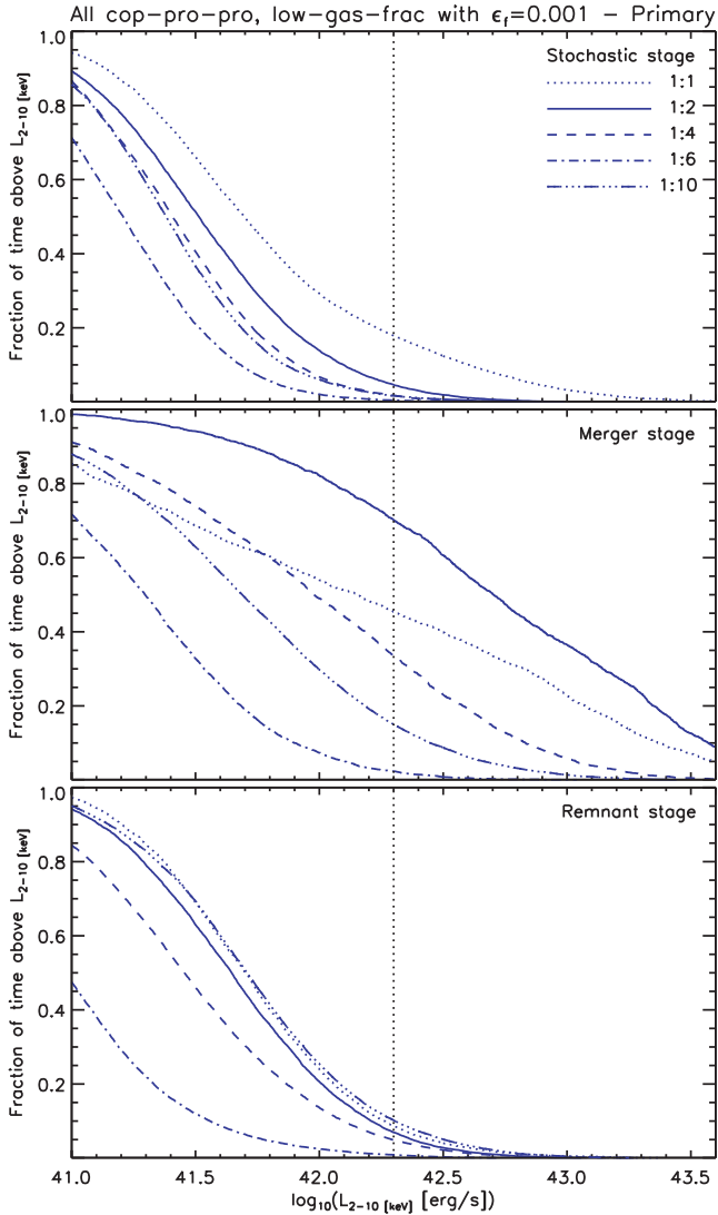
Figure 7. Fractional cumulative time above a given luminosity – coplanar, prograde–prograde mergers with low gas fraction and \epsilon_f = 0.001 – primary BH. Same as Fig. 5. Top panel: fractional cumulative time for the stochastic stage, for the primary BH of the 1:1 (dotted), 1:2 (solid), 1:4 (dashed), 1:6 (dash–dotted), and 1:10 (triple–dot–dashed) merger. Middle panel: same as the top panel, but for the merger stage. Bottom panel: same as the top panel, but for the remnant stage.
