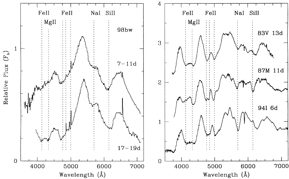
Figure 3. Left: SN 1998bw on days 7 to 11 and days 17 to 19. Right: Spectra of other Ic SNe at similar epochs. All spectra have been corrected for the redshift of the parent galaxy. Positions of median line centres shifted by -10\,000\text{ km s}^{-1} relative to rest are shown in both panels for the Fe II multiplet \lambda 4274 , Mg II \lambda 4481 , Fe II \lambda\lambda 4923, 5018, 5169 , Na I \lambda\lambda 5890, 5896 and Si II \lambda\lambda 6347, 6371 .
