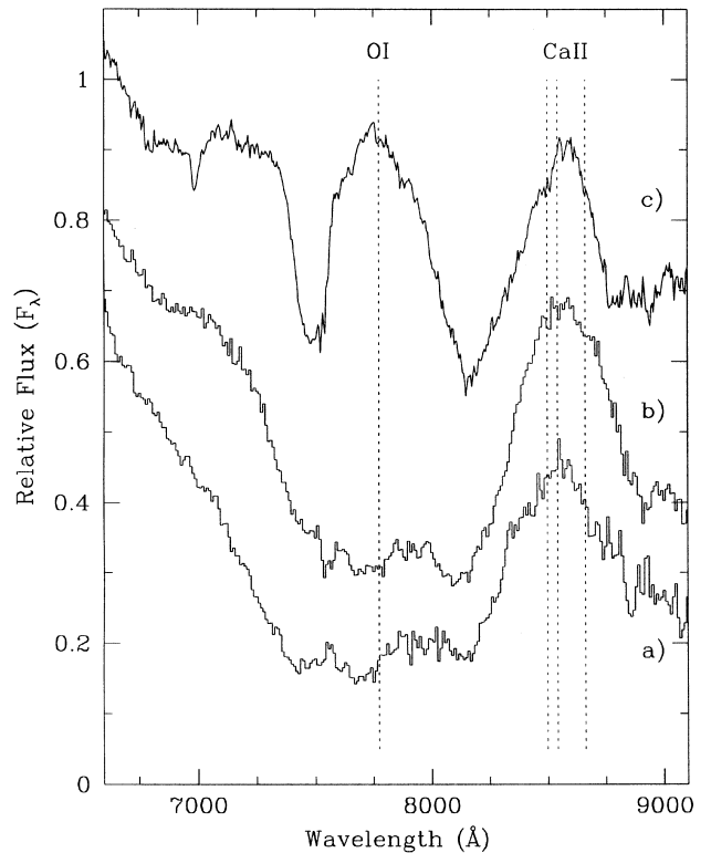
Figure 6. The 7000 to 9000 Å region of Ic SNe spectra is dominated by the O I \lambda 7774 multiplet and Ca II \lambda\lambda 8498, 8542, 8662 (rest wavelengths are shown). These lines are blended in SN 1998bw on day 11 (a) and day 19 (b), but are well separated in SN 1987M on day 7 (c). Note that weak residual telluric lines are present in the SN 1998bw spectra, especially around 7600 Å.
