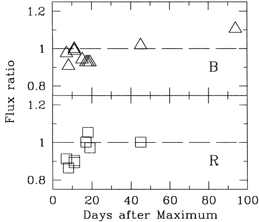
Figure 1. Comparison of B -band (top panel) and R -band (bottom panel) spectrophotometry from the corrected spectra with published photometry. Both bands show scatter with \sigma = 6 per cent.
