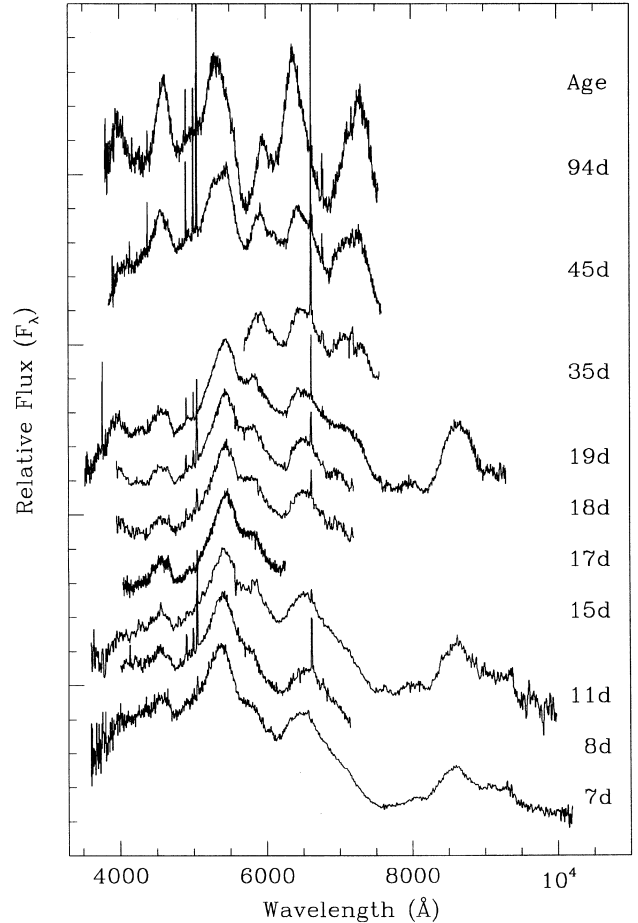
Figure 2. Spectral evolution of SN 1998bw. Ages are shown relative to date of visual maximum, 1998 May 12. Spectra have been normalized by the V -band photometry (see text) and offset in flux for the purpose of comparison.
