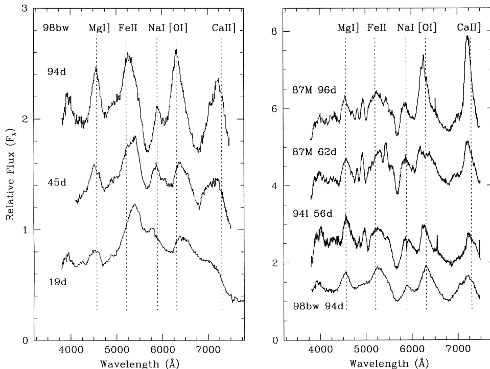
Figure 4. Left: Comparison of spectra taken on days 19, 45 and 94. Spectra have been normalized as in previous plots and shifted to rest at z = 0.0086 . In addition, nebular lines from nearby H II regions have been removed. Right: Spectra of other Ic SNe at similar epochs. Median rest wavelengths are indicated for Mg I \lambda 4571 , Fe II \lambda 5215 , Na I \lambda\lambda 5890, 5896 , [O I] \lambda\lambda 6300, 6363 and Ca II \lambda\lambda 7298, 7323 .
