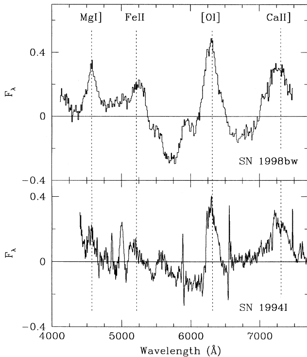
Figure 5. Top: Difference between spectra of SN 1998bw observed on day 45 and 94, after scaling by the V-band photometry. Narrow lines from nearby H II regions have been removed. Excess emission from broad nebular lines are visible as SN 1998bw enters the supernebular phase. Bottom: Difference between day 36 and 56 spectra of SN 1994I.
